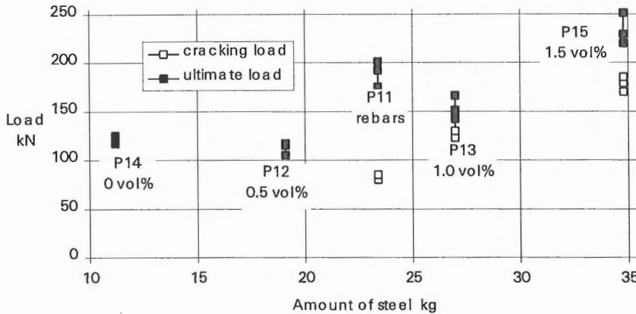
Fig. 10. Beam test results as a function of the total amount of reinforcement steel.
