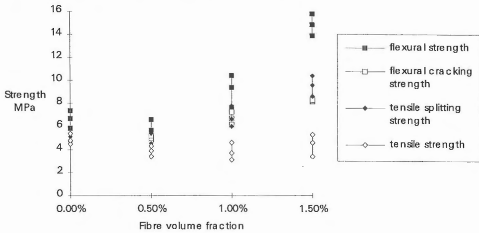
Fig. 3. Determined strength values as a function of the fibre content; the minimum, maximum and average values are presented.
