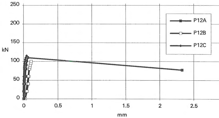
Fig. 6. Average deflections of flange; beam P12A...C with a fibre content of 0.5 %.
