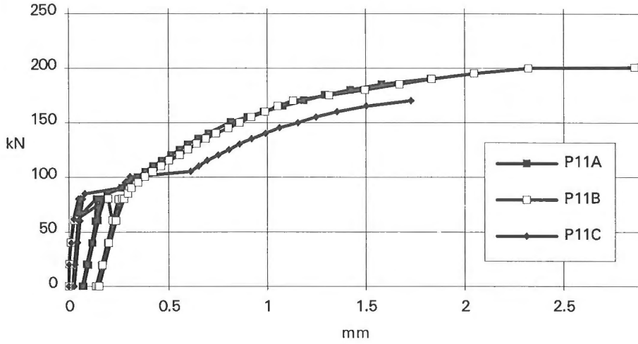
Fig. 5. Average deflections of flange; beam P11A...C with normal stirrups.
