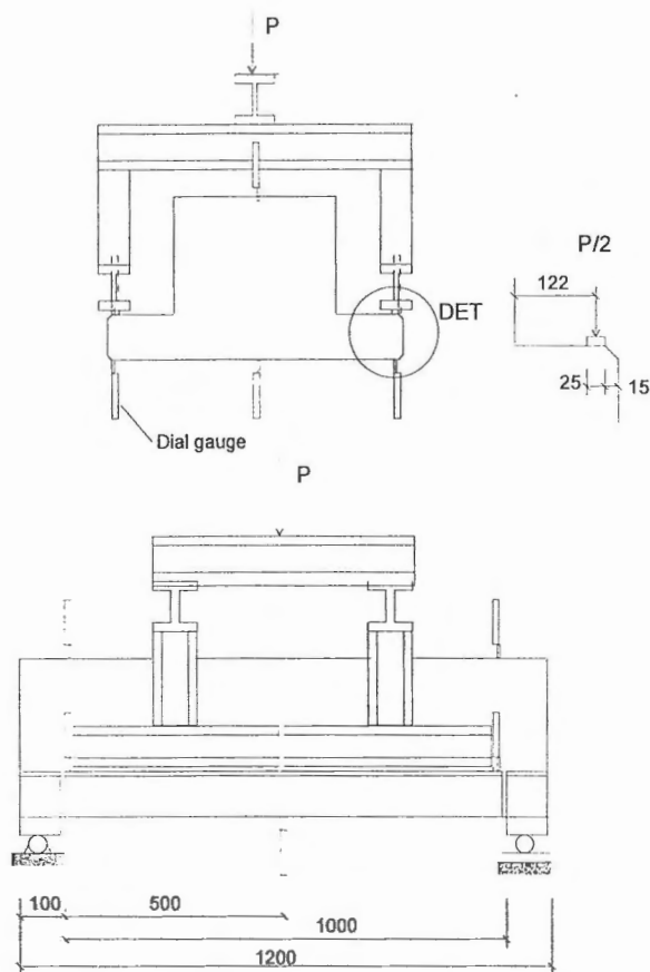
Fig. 1. Test arrangements
