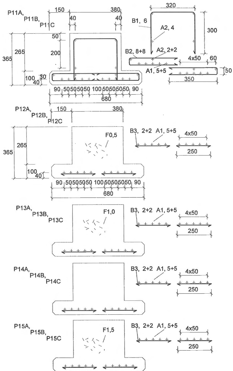
Fig. 2. Cross-sections of the beams.
