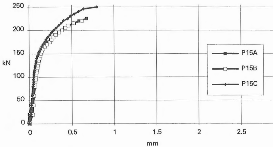
Fig. 9. Average deflections of flange; beam P15A...C with a fibre content of 1.5 %.
