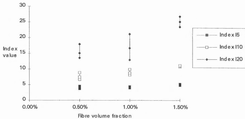
Fig. 4. Toughness index values ( I_5 , I_{10} , I_{20} ) as a function of the fibre content; the minimum, maximum and average values are presented.
