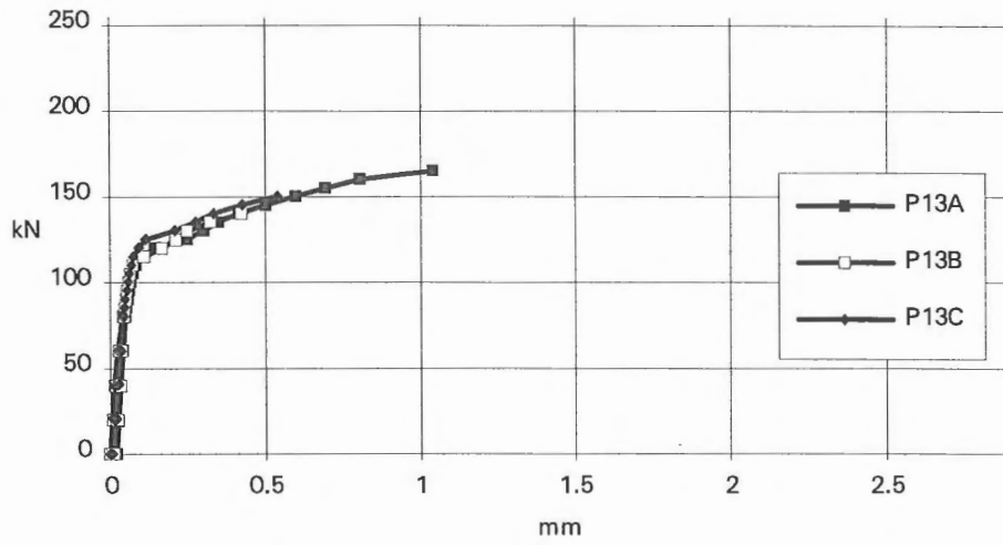
Fig. 7. Average deflections of flange; beam P13A...C with a fibre content of 1 %.
